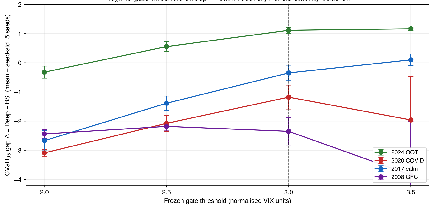
Regime-gate threshold sweep — calm-recovery / crisis-stability trade-off
